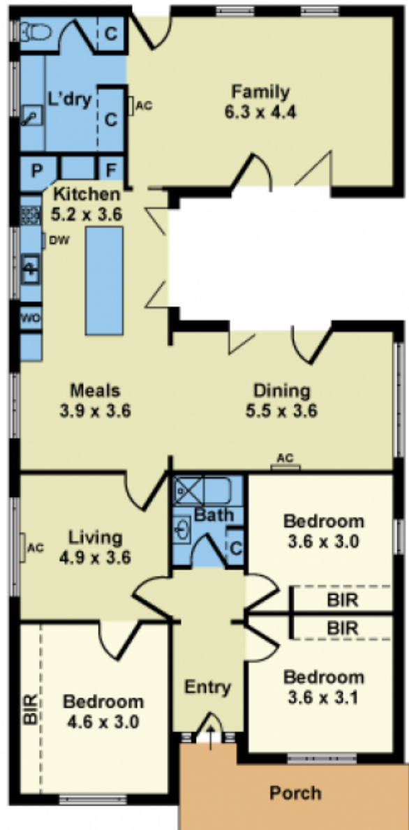
FLOOR PLAN
