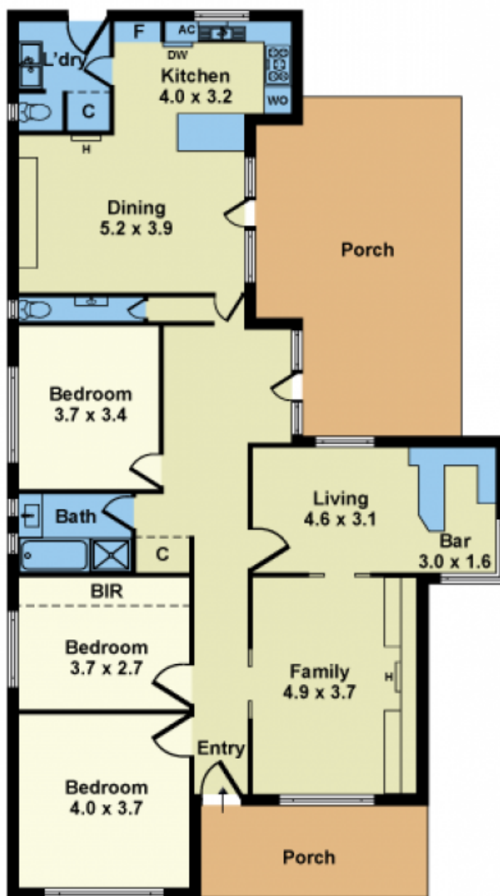
FLOOR PLAN
