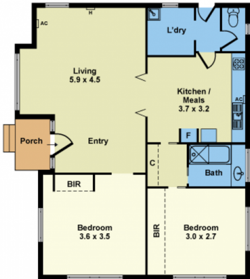
FLOOR PLAN
