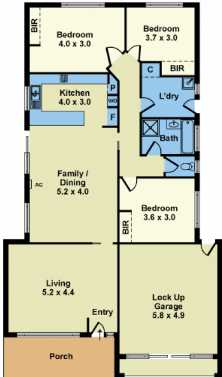
FLOOR PLAN
