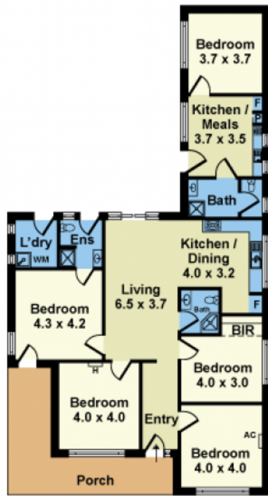
FLOOR PLAN
