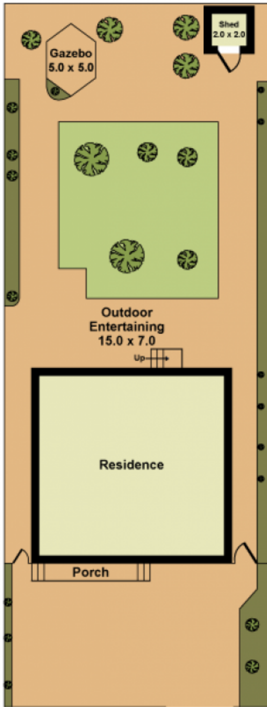
SITE PLAN
