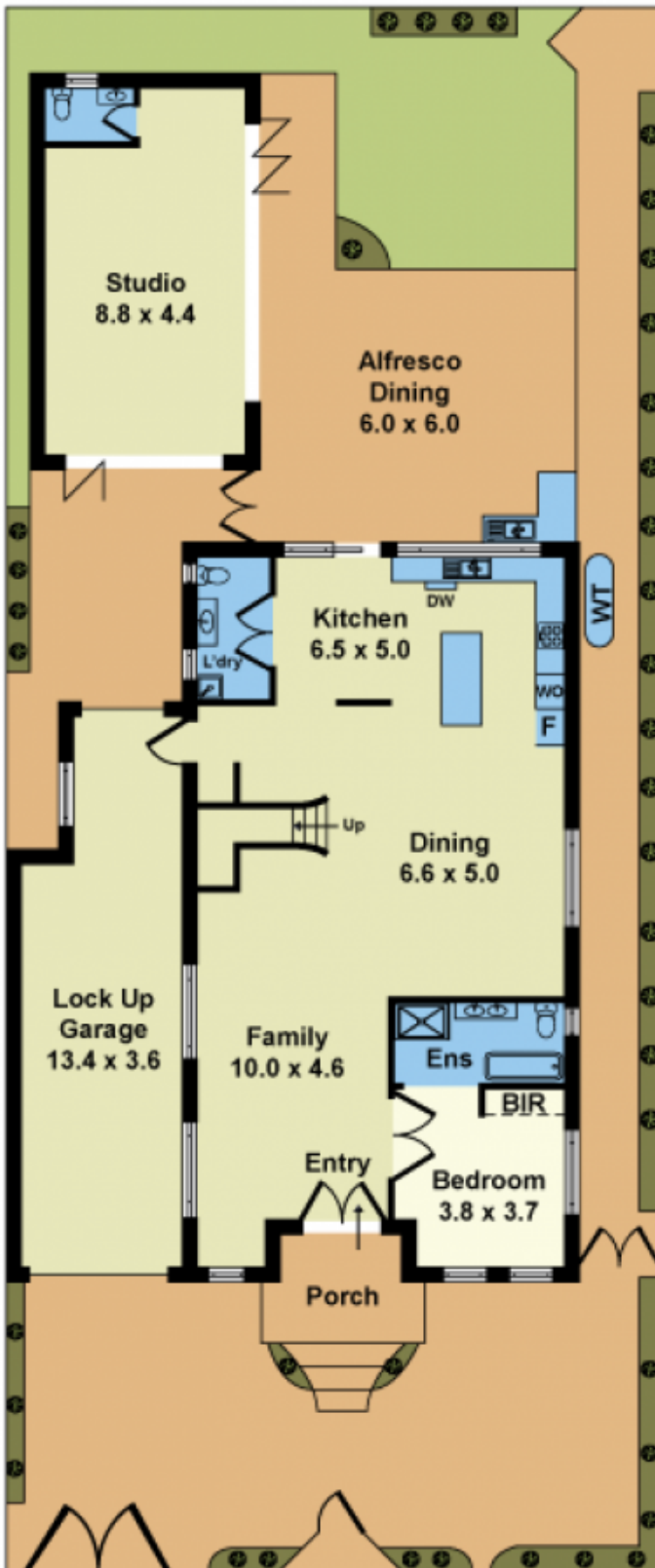
GROUND FLOOR
