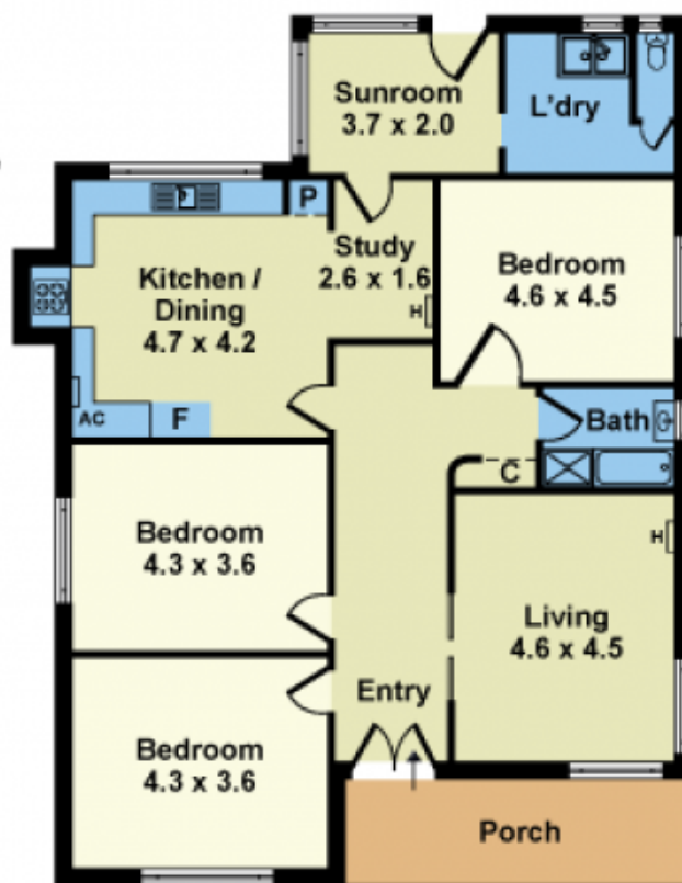
FLOOR PLAN
